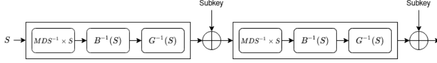
Figure 3: A CHAGHRI encryption round function
