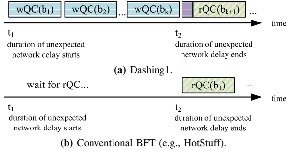
Figure 5: The way how Dashing1 and a regular BFT handle unexpected network delays, respectively.
