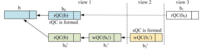
Figure 8: Challenge of integrating strong certificates in Dashing2.
