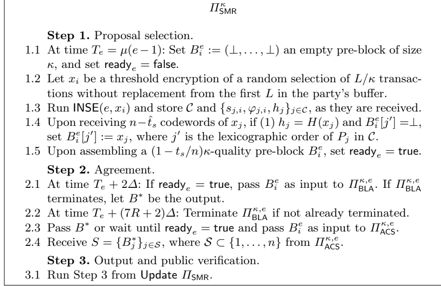
Fig. 7. SMR protocol with static security for party P_{i \in \{1, \dots, n\}} .
