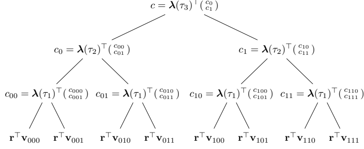
Fig. 4: Demonstration of the tree structure of a commitment. Leaf nodes are commitments to k -dimensional vectors for an arbitrary vector commitment scheme. Each node is a commitment to its children under a Lagrange based key. The message space of the scheme is k \cdot 2^3 .
