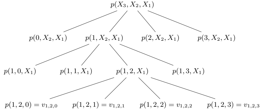
Fig. 3: Tree structure for polynomials in 3 variables with individual degree at most 3. The dimension of the committed vectors with these parameters is 4^3 = 64 . We follow the path until we reach the leaves prefixed with (1, 2). Note that each polynomial is an encoding of the leaves of the sub-tree it defines.
