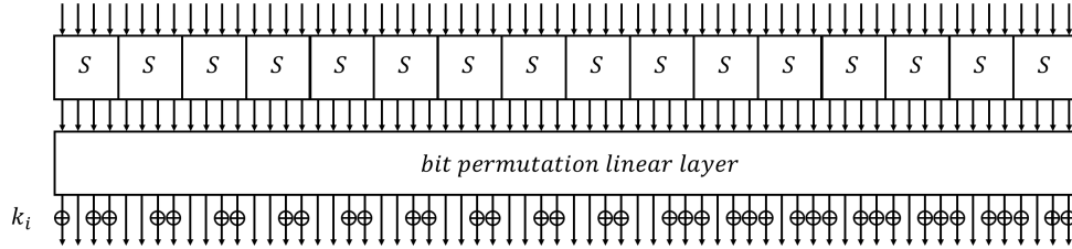
Figure 6: Round function of Gift-64
