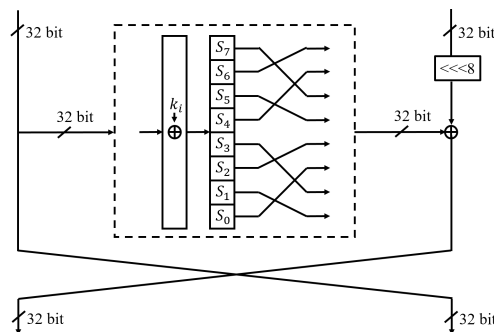
Figure 2: Round function of LBlock
