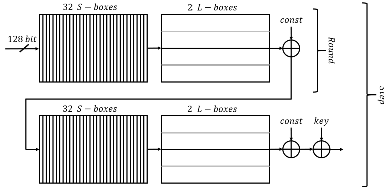
Figure 7: Round and Step of Clyde-128
