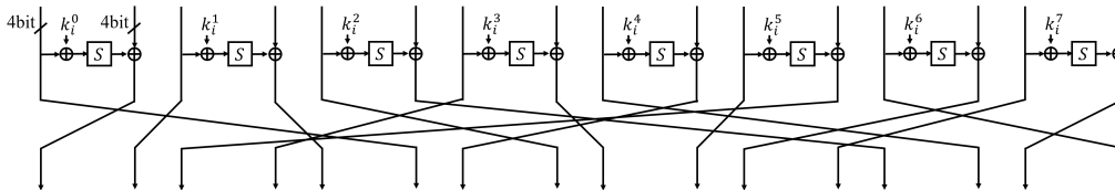
Figure 3: Round function of TWINE
