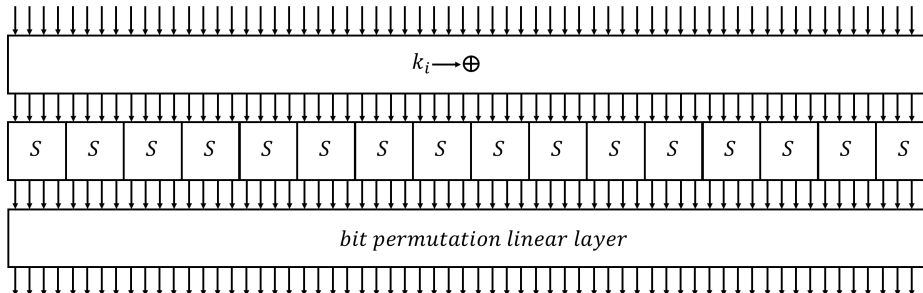
Figure 5: Round function of PRESENT
