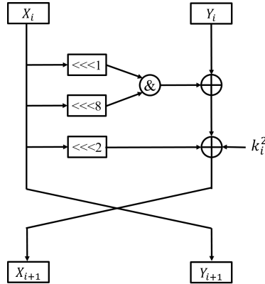
Figure 4: Round function of SIMON
