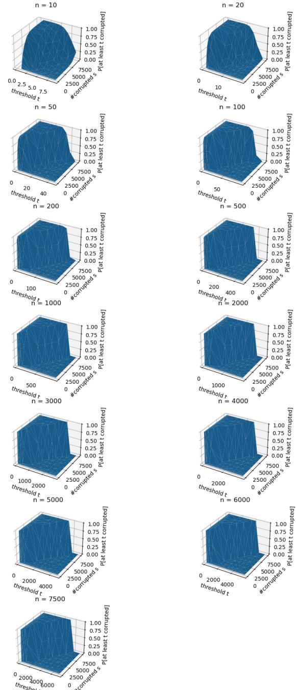
Figure 11: Visualisation of probabilities of bad event for |\mathcal{P}| = 10000 and various parameter values
