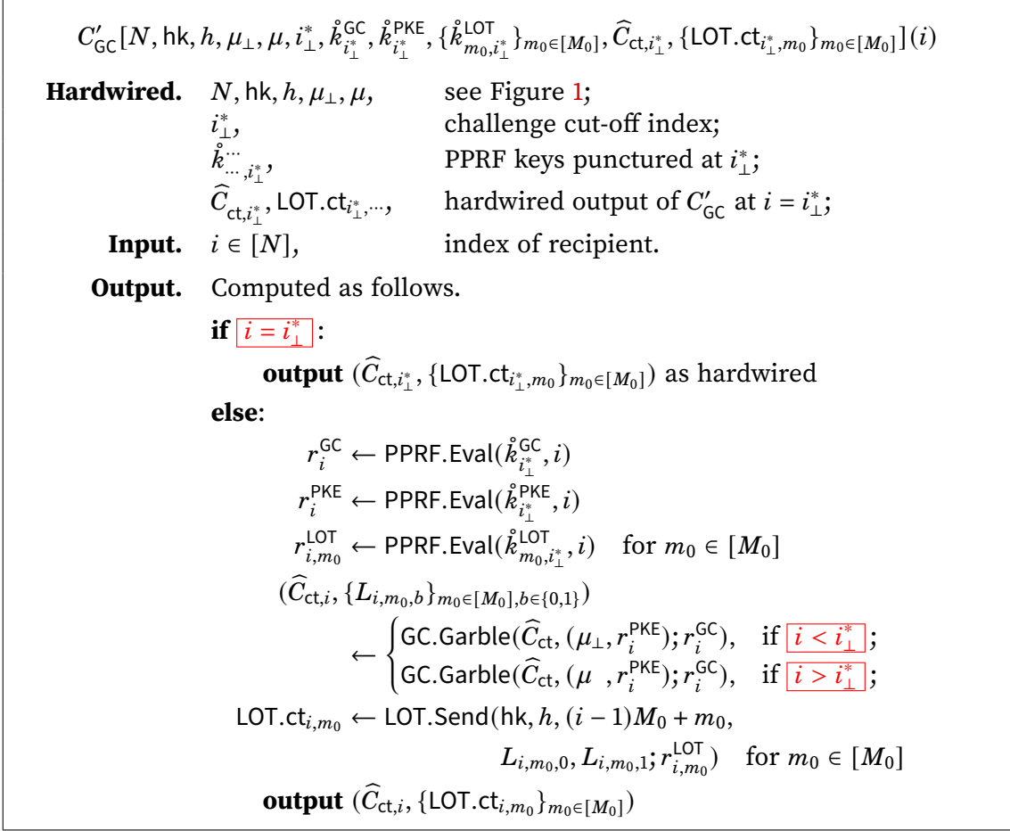
Figure 2. The circuit C'_{GC} in the proof of Theorem 4.
