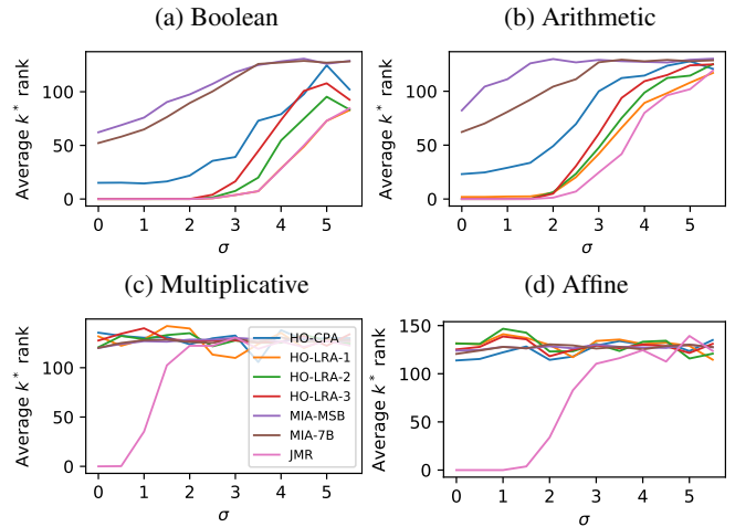
FIGURE 2: Guessing entropies versus standard deviation of the noise for the considered third-order attacks.
