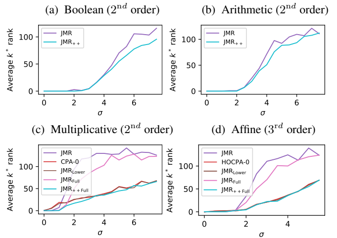
FIGURE 3: Guessing entropies for the improved JMR attacks, using the GMM theory, and for (HO)CPA-0.
