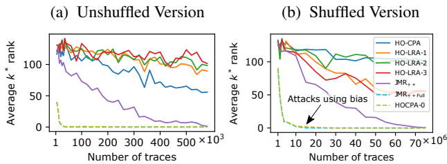
FIGURE 4: Comparison of different attacks' guessing entropies on the secured ANSSI's AES
