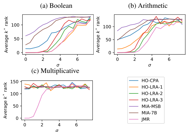
FIGURE 1: Guessing entropies versus standard deviation of the noise for the considered second-order attacks.
