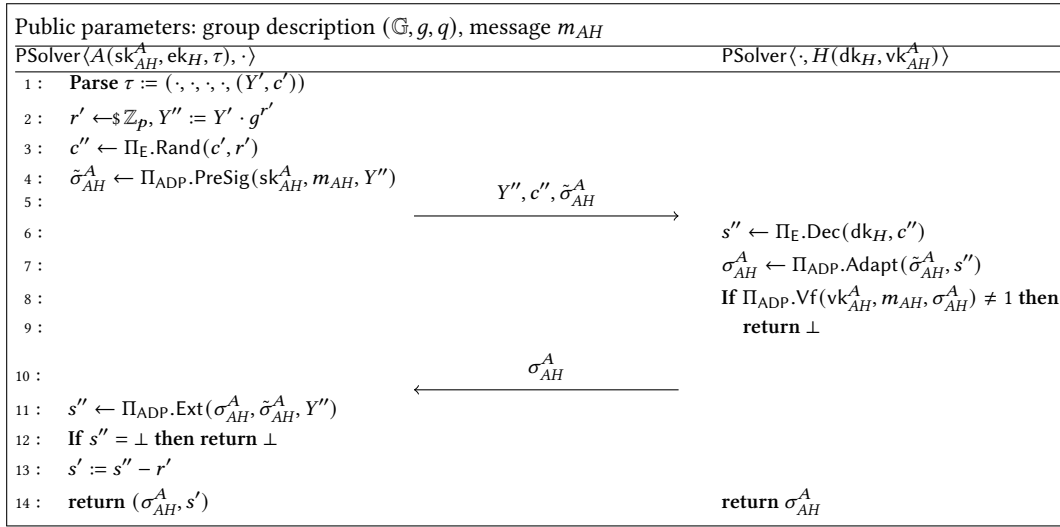
Figure 13: Puzzle solver protocol of A^2L
