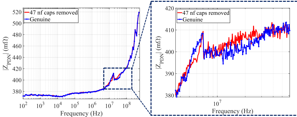
Figure 7: The mean of 105 impedance profile measurements for removing 47 nF capacitors from the board over the frequency band of 100 Hz - 588 MHz. The right-side figure shows the zoomed-in view of the bandwidth with the most deviation from the mean graph.
