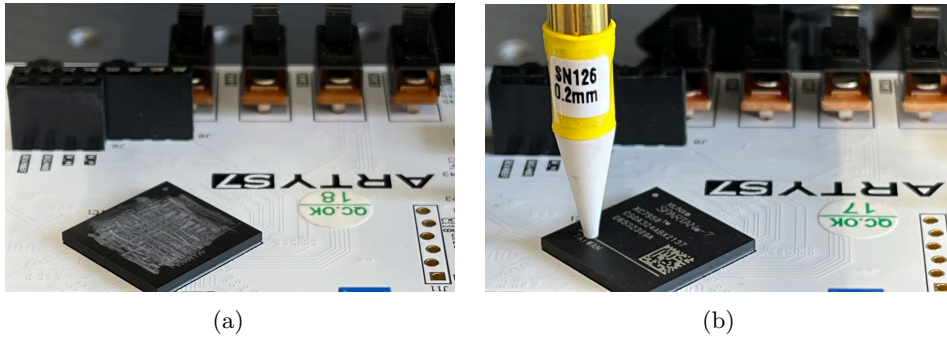
Figure 8: Devices under attack (a) Polished FPGA package (b) Placing an EM probe on top of the FPGA package.
