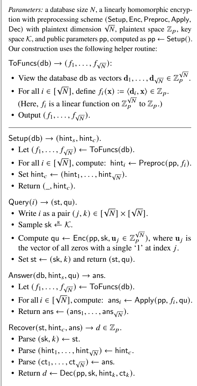
Figure 13: The SimplePIR protocol, expressed in terms of linearly homomorphic encryption with preprocessing.
