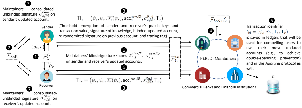
Fig. 4. Payment Protocol
