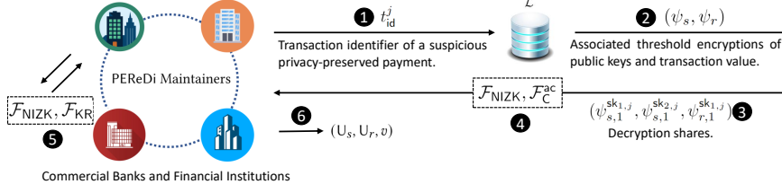
Fig. 5. Privacy Revocation Protocol
