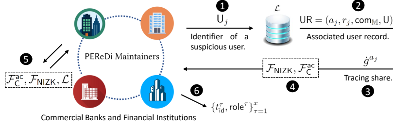
Fig. 6. Tracing Protocol
