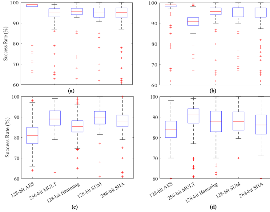
Figure 3: SR of Goblin for 1000 randomly chosen inputs given to GC garbled by TinyGarble [101] with (a) free-XOR, (b) half-gate optimizations, (c) JustGarble [53], and (d) Obliv-C [112].
