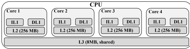
Figure 2: Intel core-i7 cache architecture [84].
