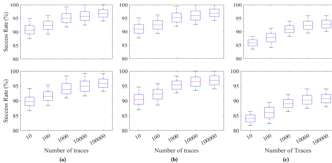
Figure 9: SR of Goblin against 128-bit (a) SUM, (b) Hamming, and (c) MULT. CPU cycle traces captured from 10-100,000 randomly chosen inputs when JG is disabled. (Top: TinyGarble [100] with only free-XOR, Bottom: with half-gate optimization).
