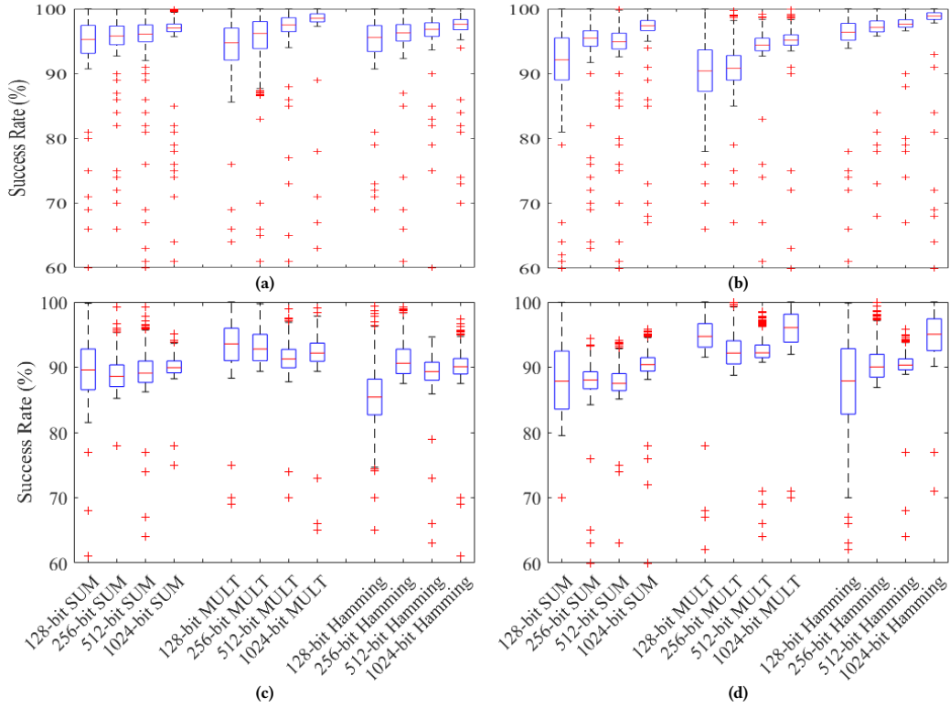
Figure 4: SR of Goblin against benchmark functions for a range of input bits garbled by TinyGarble [100] with (a) only free-XOR optimization, (b) half-gate protocol, (c) JustGarble [53], and (d) Obliv-C [112] for 1000 randomly chosen inputs.
