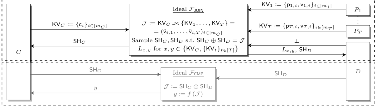
Fig. 2. Ideal functionality \mathcal{F}_{\text{DPMC}} of private join for compute is composed by \mathcal{F}_{\text{JOIN}} and \mathcal{F}_{\text{CMP}} . Parties C and P_1, \dots, P_T provide inputs. \mathcal{F}_{\text{JOIN}} computes a left join with associated data \mathcal{J} := KV_C \bowtie \{KV_1, \dots, KV_T\} as described in Def. 3 (or alternatively Def. 4). Later on, C and D can query \mathcal{F}_{\text{CMP}} with their secret shares ( SH_C and SH_D ) and \mathcal{F}_{\text{CMP}} will reconstruct \mathcal{J} := SH_C \oplus SH_D and compute y := f(\mathcal{J}) and send it to party C . Party D gets leakage L_{x,y} , where x and y are the sets of any party in \{KV_C, KV_1, \dots, KV_T\} .
