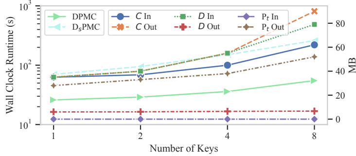
Fig. 9. Wall clock time for DPMC and D_s PMC. DPMC network traffic for each party C , D , and P_t with an increasing number of keys per row for m_C = m_t = 10^5 and an intersection size of 50% of m_C .
