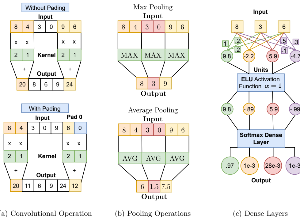
Figure 1: Convolutional Operation, Pooling Operation and Dense layers of CNN
