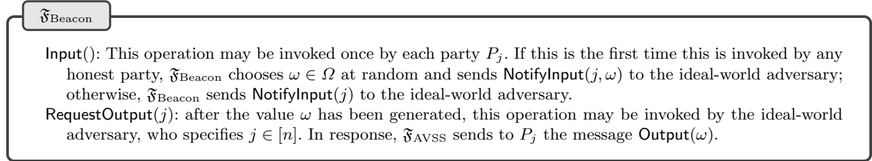
Fig. 4. The Random Beacon Functionality \mathfrak{F}_{\text{Beacon}} (parameterized by output space \Omega )
