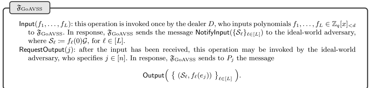
Fig. 2. The GoAVSS Ideal Functionality (parameterized by n, d, L, E (which defines \mathbb{Z}_q ), \mathbf{e} , and D )
