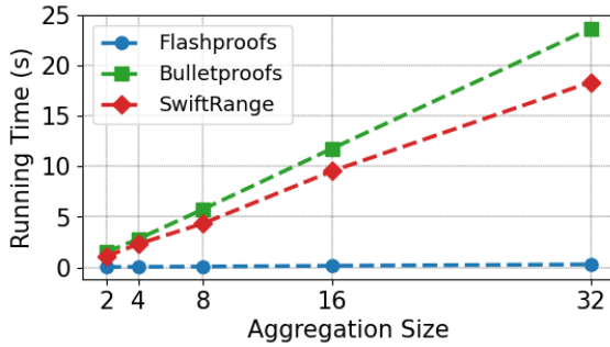
(a) The proving running time in seconds.
