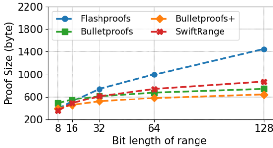
(a) The proof size of single range arguments.
