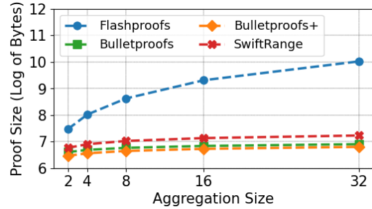
(b) The proof size of aggregate range arguments.
