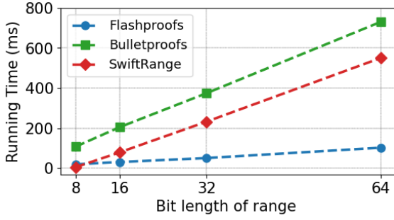
(a) The proving running time in milliseconds.
