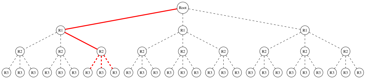
Figure 3: 3-round IOP tree with a highlighted completable partial transcript. In this figure, the highlighted path through the tree ends in the second round with node R2, and the hanging tree (with dashed red edges) at R2 represents the tree that completes the partial transcript.
