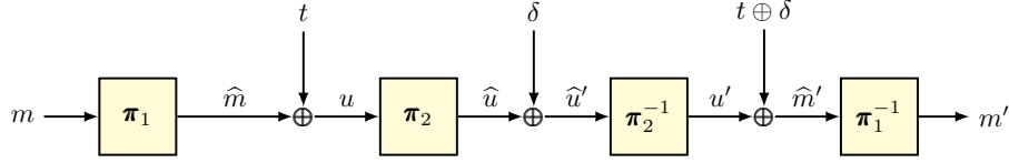
Fig. 1.2: TNT with final-block cancellation.
