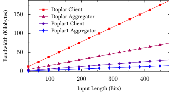
Figure 8: The total number of kilobytes sent by each party, per report, for various input lengths.
