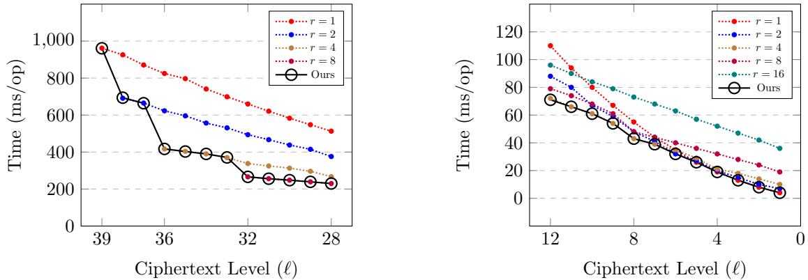
Fig. 1: Performance of key-switching operation when N = 2^{16} . r = 1, 2, 4, 8, 16 stands for the previous method with each r , and Ours stands for our new method.
