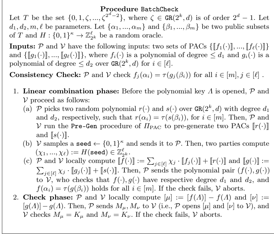
Fig. 6: Procedure for checking the \tau -consistency of polynomial evaluations for two sets of PACs.
