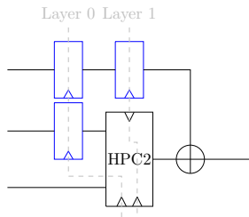
Figure 1: Example of a masked pipelined circuit as a composition of gadgets and masked registers.
