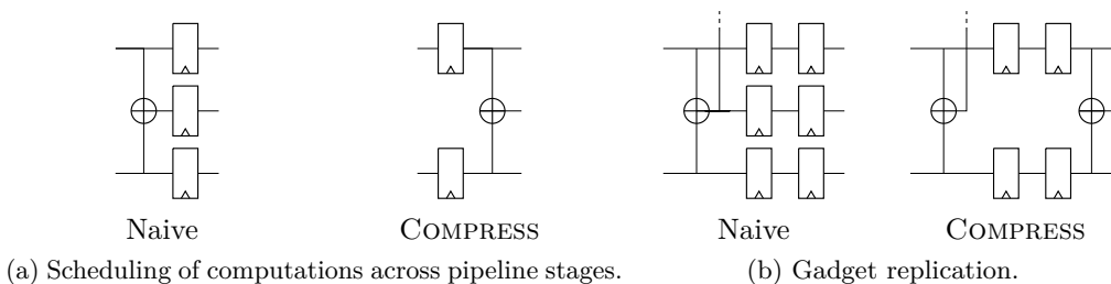
Figure 4: Examples of COMPRESS optimization of pipeline registers (registers and \oplus represent sharewise gadgets, wires represent sharings).
