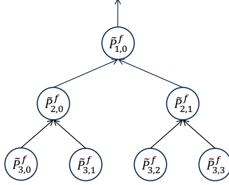
Figure 4: The malicious provers constructed as in Construction 5.11 and Construction 5.12 when transcript depth is at most 3.
