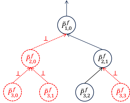
Figure 6: The behavior of the malicious provers for the transcript in Fig. 5. The provers circled with red dashed lines output \perp .
