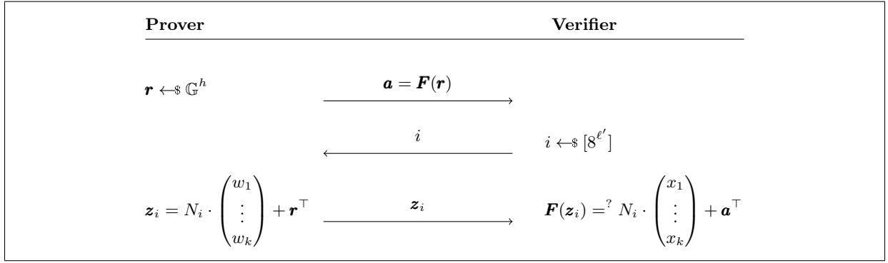
Fig. 12. \Sigma -protocol from Theorem 5
