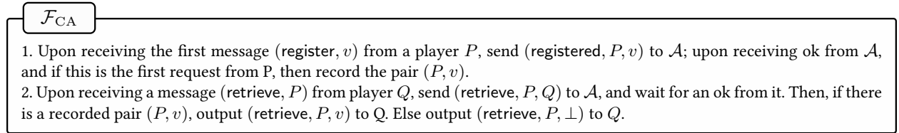
Figure 6: The certification authority functionality: \mathcal{F}_{CA} .
