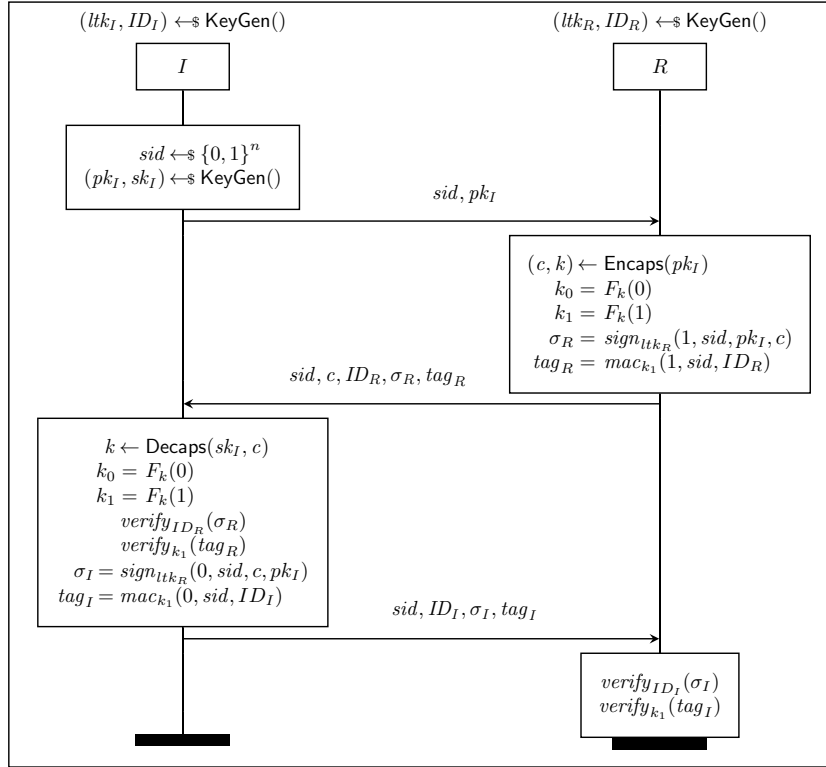
Figure 10: The \Sigma'_0 -protocol introduced by [39].
