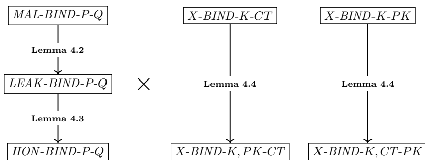
Figure 11: Restricted hierarchy of binding properties for implicitly-rejecting KEMs as X\text{-BIND-CT-K} and X\text{-BIND-CT-PK} cannot be met by any implicitly-rejecting KEM
