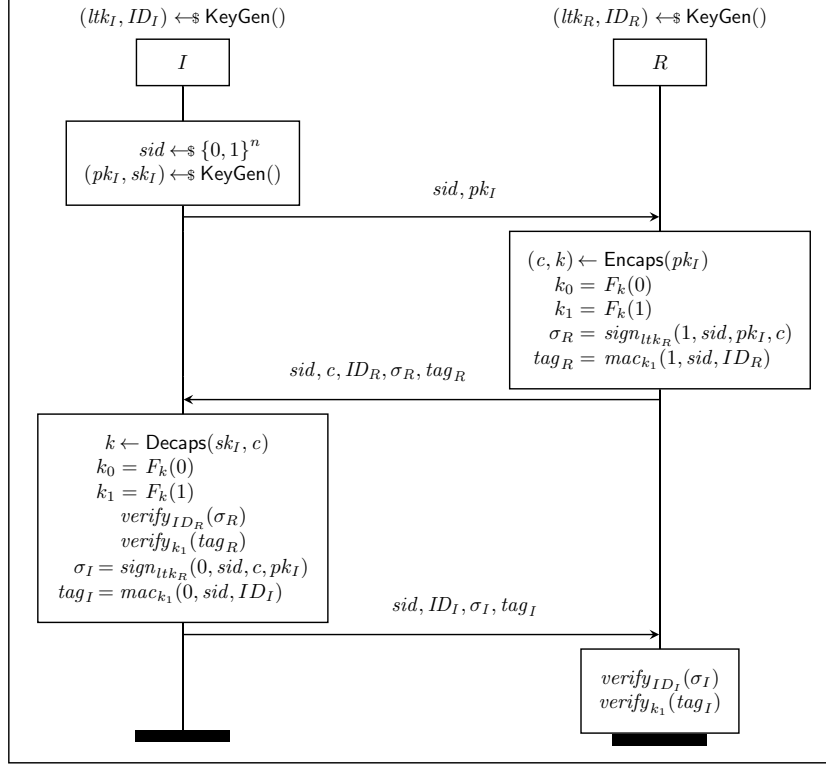
Figure 10: The \Sigma'_0 -protocol introduced by [41].
