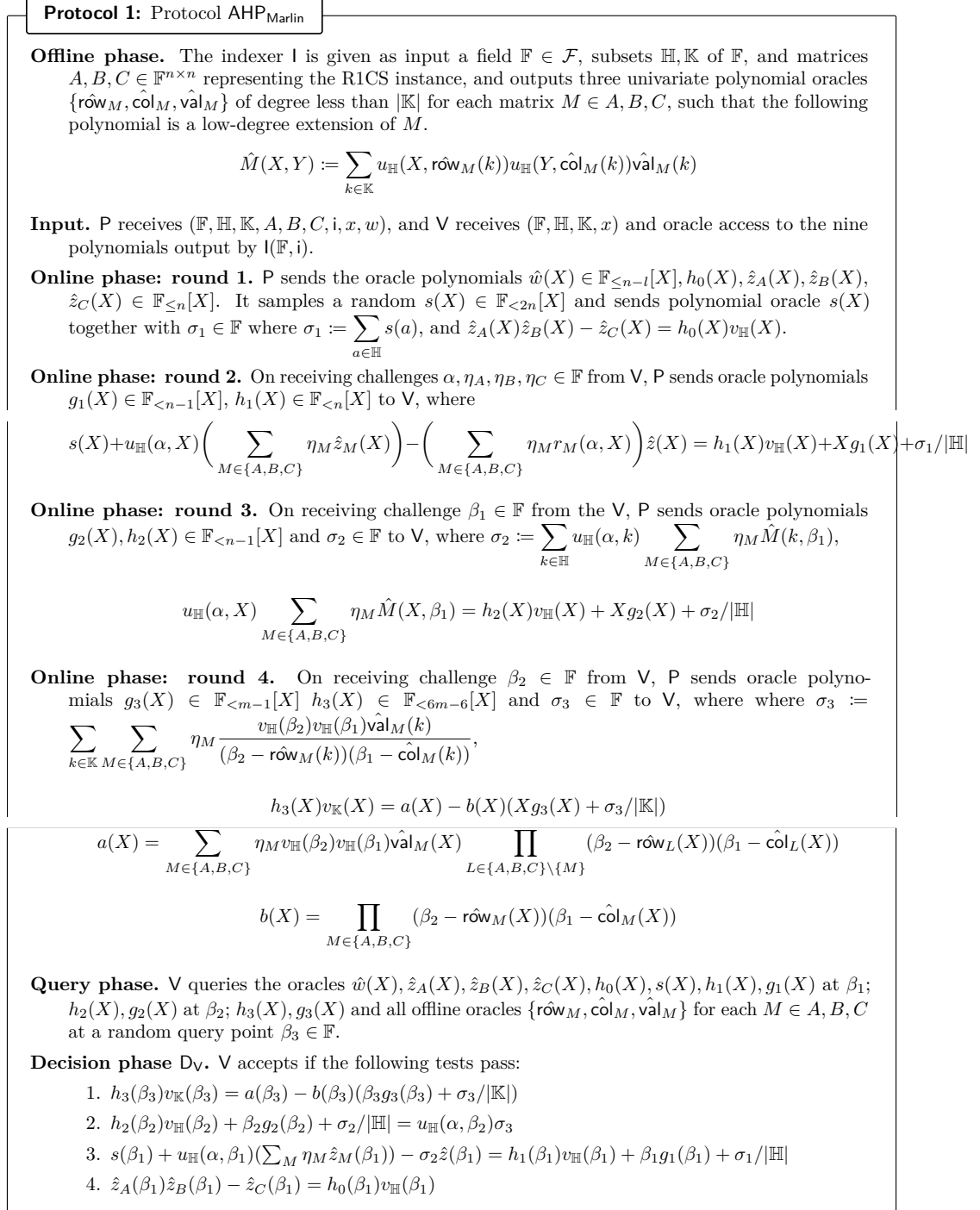
Figure 6: AHP for \mathcal{R}_{\text{R1CS}}
