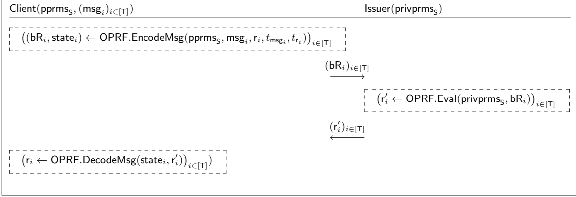
Fig. 6: Oblivious Evaluation of PRF.
