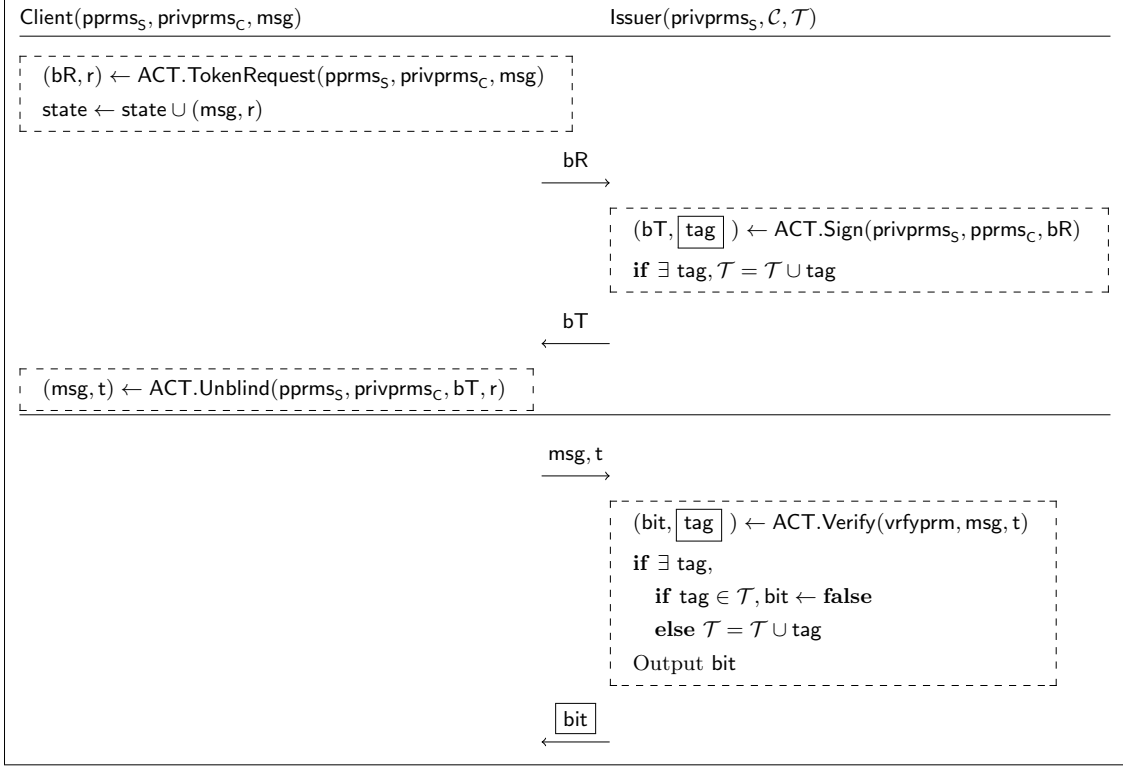
Fig. 2: Token issuance and verification for ACT (Definition 3.1).
