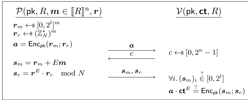
Fig. 9. \text{SigmaRangeA}_{\text{Prot}} : Amortized variant of \text{SigmaRange}_{\text{Prot}} which proves knowledge of Paillier preimage and its range for n instances, where E = w(c) , and l = \lambda + \log n + \log R - 1 .
