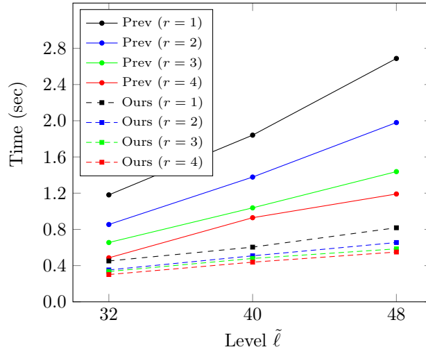
Fig. 1: Running time results of the key-switching methods with N = 2^{16} .
