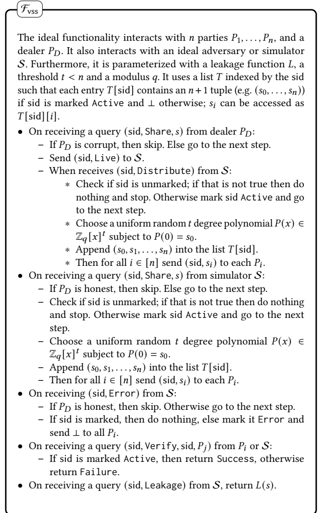
Figure 2: Ideal Functionality for VSS
