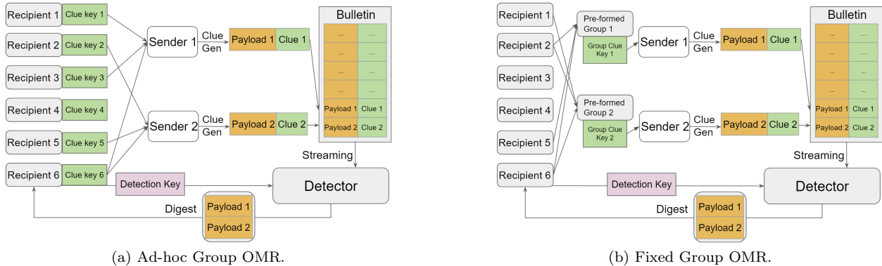
Figure 1: The high-level illustration of AGOMR and FGOMR. For AGOMR, the sender obtains the individual clue keys to form a group message. For FGOMR, individuals form a group clue key that the sender obtains.
