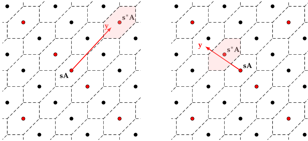
Fig. 1. Red points are in S . Possible cases of the nearest point to \mathbf{y} . The left panel shows that the closest point to \mathbf{y} is on S , but the right panel shows that the closest point to \mathbf{y} is clearly not on S
