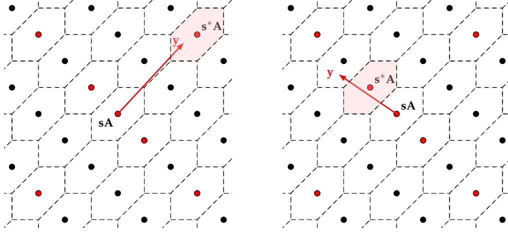
Fig. 1. Red points are in S . Cases of the nearest point to y . The left panel shows that the closest point to y is on S , but the right panel shows that the closest point to y is clearly not on S
