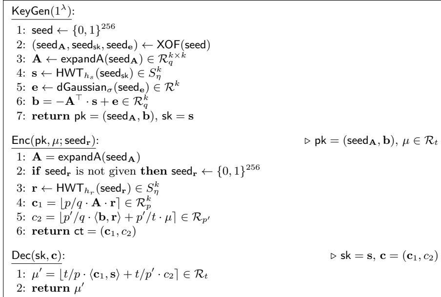
Fig. 2: Description of SMAUG.PKE
