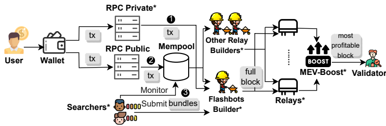
Fig. 9: Flashbots transaction order flows post-PBS. ①, ② and ③ denote private, public and search order flows. * denotes entity with potential censoring power.
