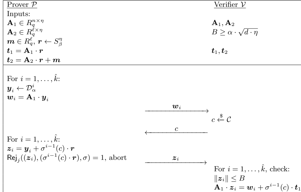
Fig. 2. Opening proof of BDLOP commitment through using our generalized rejection sampling, where j = 0, \dots, 3 .
