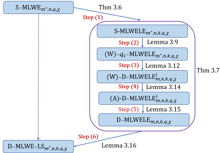
Fig. 1. Our reduction route
