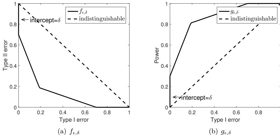
Figure 1: Examples: tradeoff functions and power functions for (\epsilon, \delta) -closeness. Here \epsilon = 1, \delta = 0.3 . (a) is the curve for f_{\epsilon, \delta} and (b) is the curve for g_{\epsilon, \delta} .
