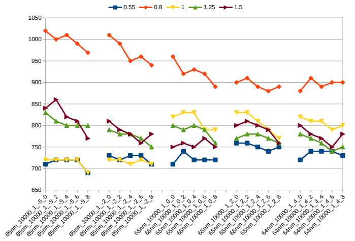
Fig. 4. NTD for AES core, in 65nm node. See also Fig. 3’s caption.
