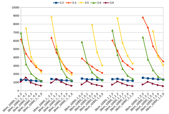
Fig. 3. NTD for AES core, in 28nm node. The legend refers to reference timing constraints in ns. For reading the naming scheme of different cases listed on the x-axis, please refer back to Sec. IV-A. Any missing data point indicates that CPA could not succeed with 10,000 traces.
