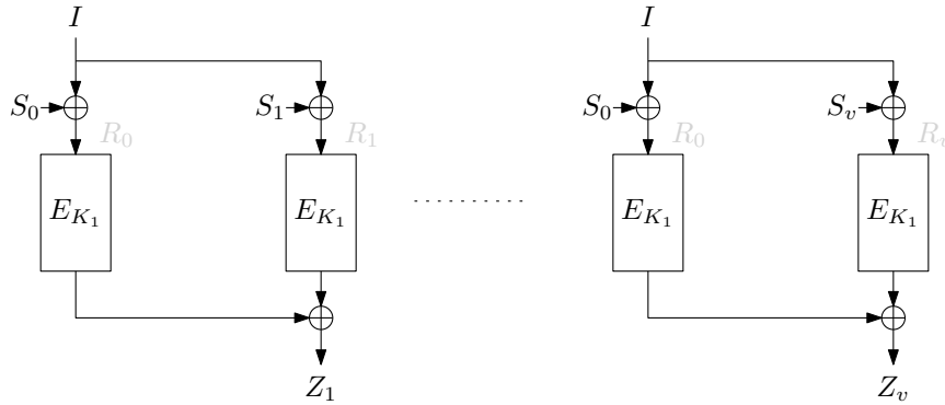
Fig. 2: The \widetilde{XORP}[v] construction. Here, S_j = E_{K_2}(B \parallel W \parallel c \parallel j) of (8). The parameters R_j will be used of the proof of Theorem 2 in Section 6 .
