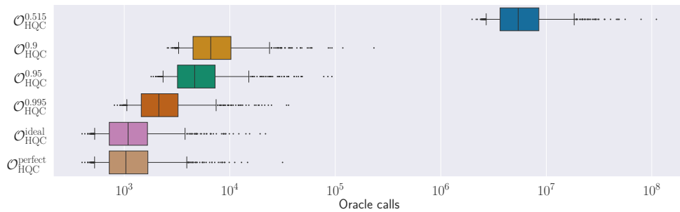
Figure 9: Oracle call requirements for attacking HQC-128 under various oracle accuracies, with whiskers representing the 5th and 95th percentile. We performed 1 000 simulated attacks per oracle accuracy.
