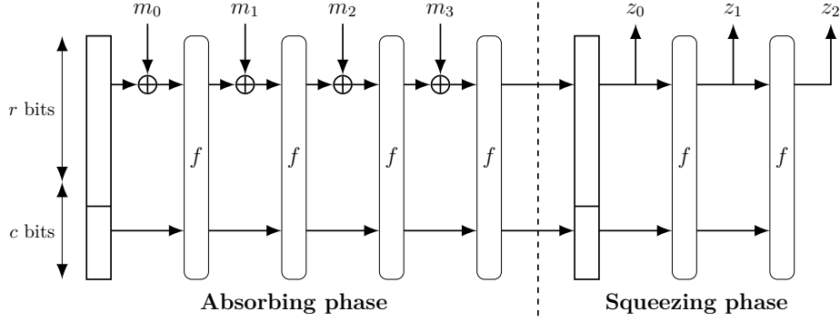
Figure 1: Visualization of the sponge construction, figure by [Jea16].
