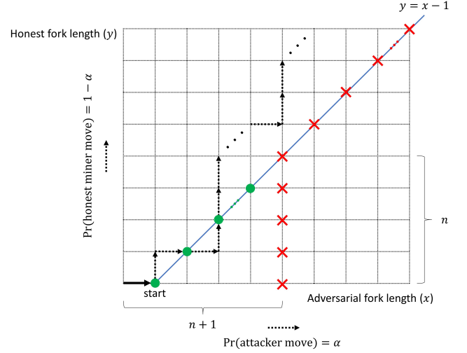
Fig. 13. Chain race representation
