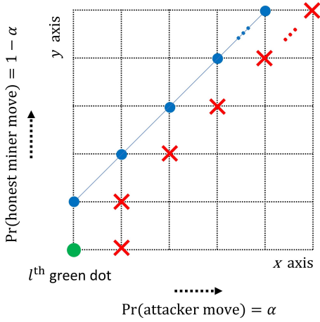
Fig. 12. The mining path starting at (0, 0) and never reaching the line y = x at x \geq 1
