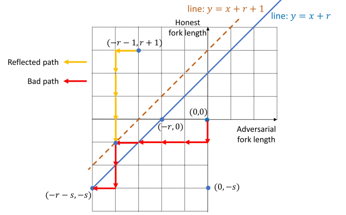
Fig. 7. Mining path representation
