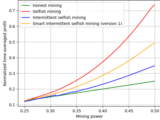
Fig. 1. Time-averaged profit under the Bitcoin’s DAM
