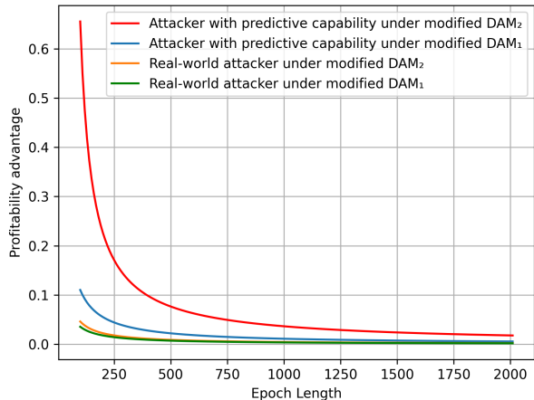
Fig. 11. The profitability advantage of strategy \pi^{\text{SM-OEA}} under the modified DAM
