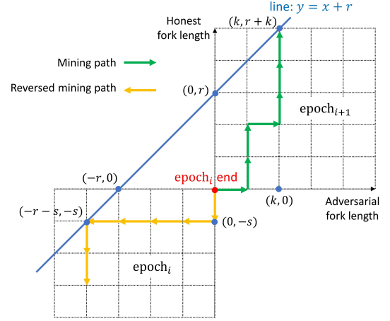
Fig. 8. Mining path representation
