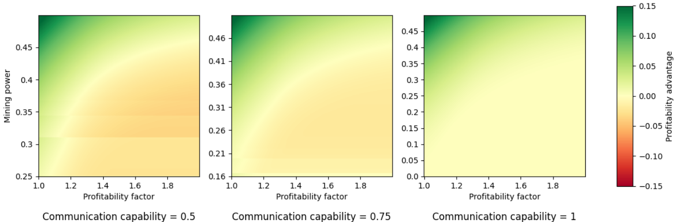
Fig. 3. Profitability advantage of SISM2 under \text{DAM}_2^{\text{modified}}
