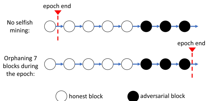
Fig. 10. The effect of selfish mining during the epoch on the end of the epoch
