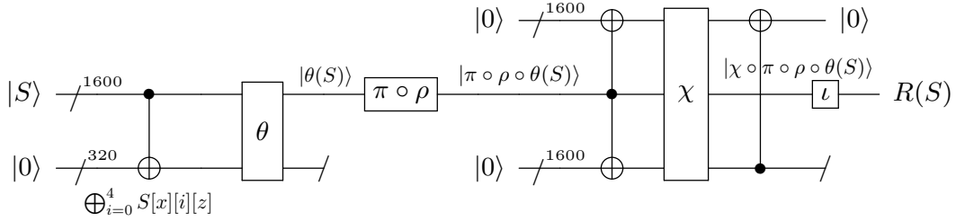
Figure 7: Out-of-place round implementation for SHA-3 (Ours).
